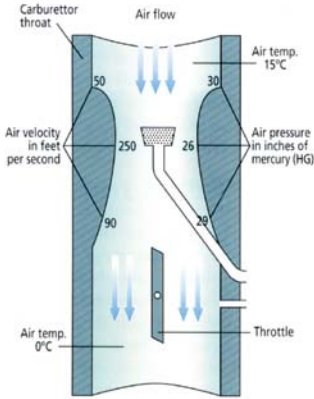
Simplified views of a venturi showing changes in air velocity and temperature. These vary in relation to changes in throttle opening and engine rpm.
