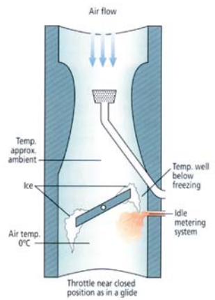
The risk of serious carburettor icing is greatest at lower or idle power settings. When carrying out prolonged glides, the engine must be warmed regularly to provide sufficient exhaust heat to the hot-air heat exchanger.
