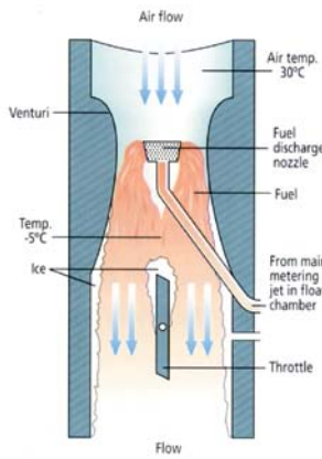
Float-type carburettors have a fuel discharge nozzle located in the venturi. Venturi action plus cooling effect of fuel vaporisation can reduce mixture temperatures markedly.
