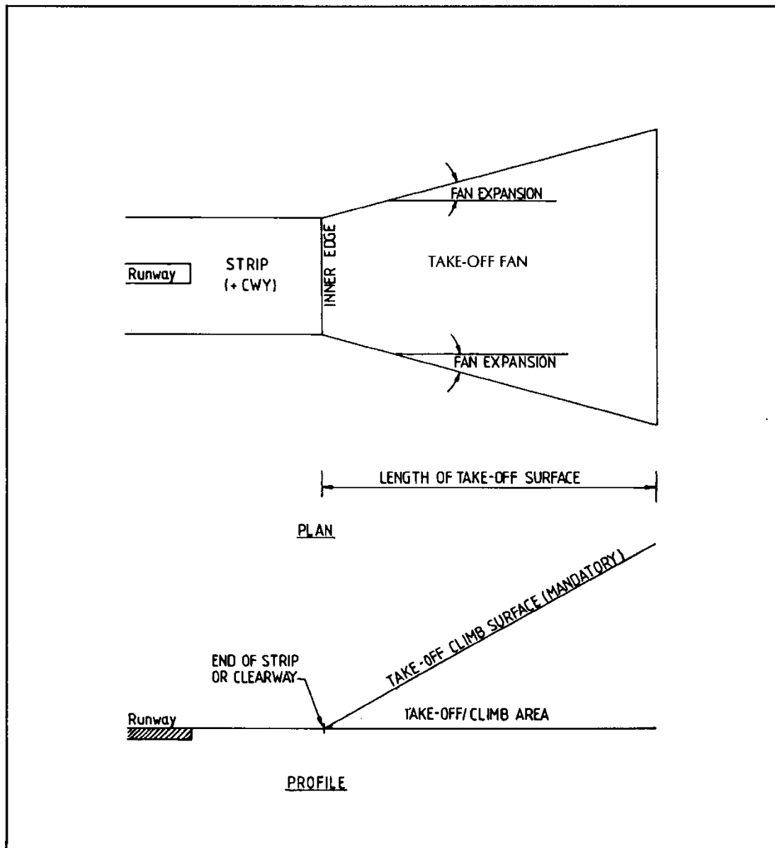
Figure 4-5. Take-off climb area and surface
