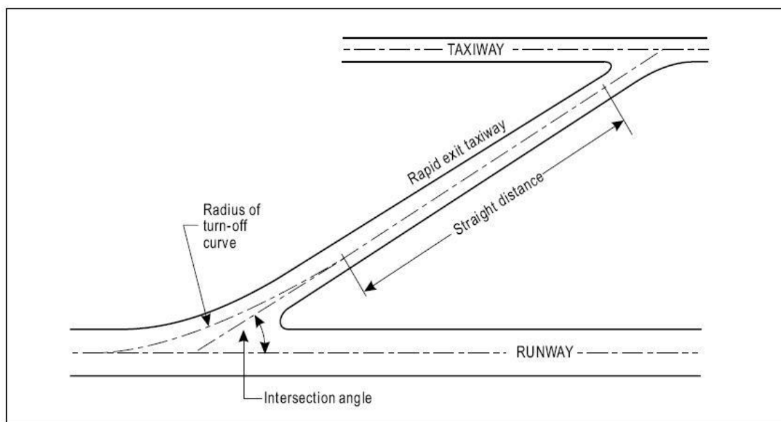
Figure 3-3. Rapid exit taxiway
