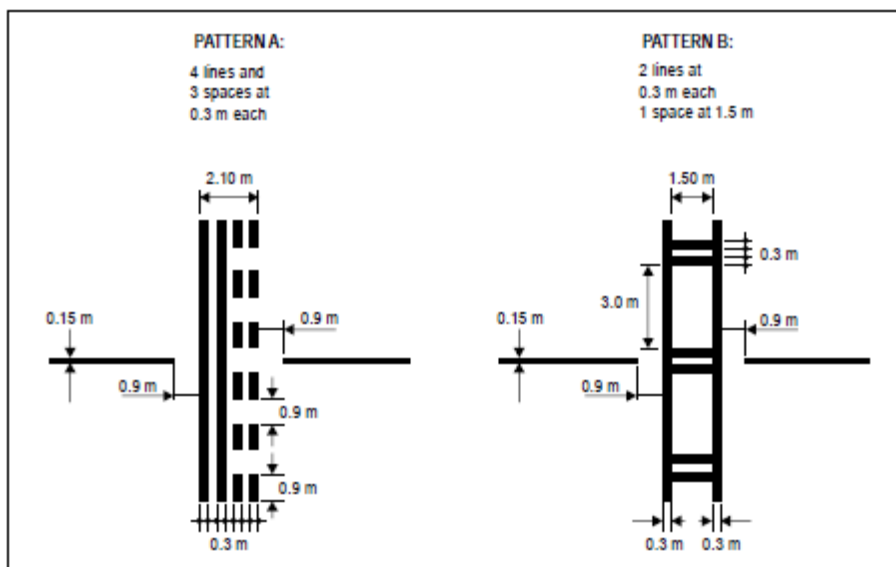
Figure 5-8. Runway-holding position markings
