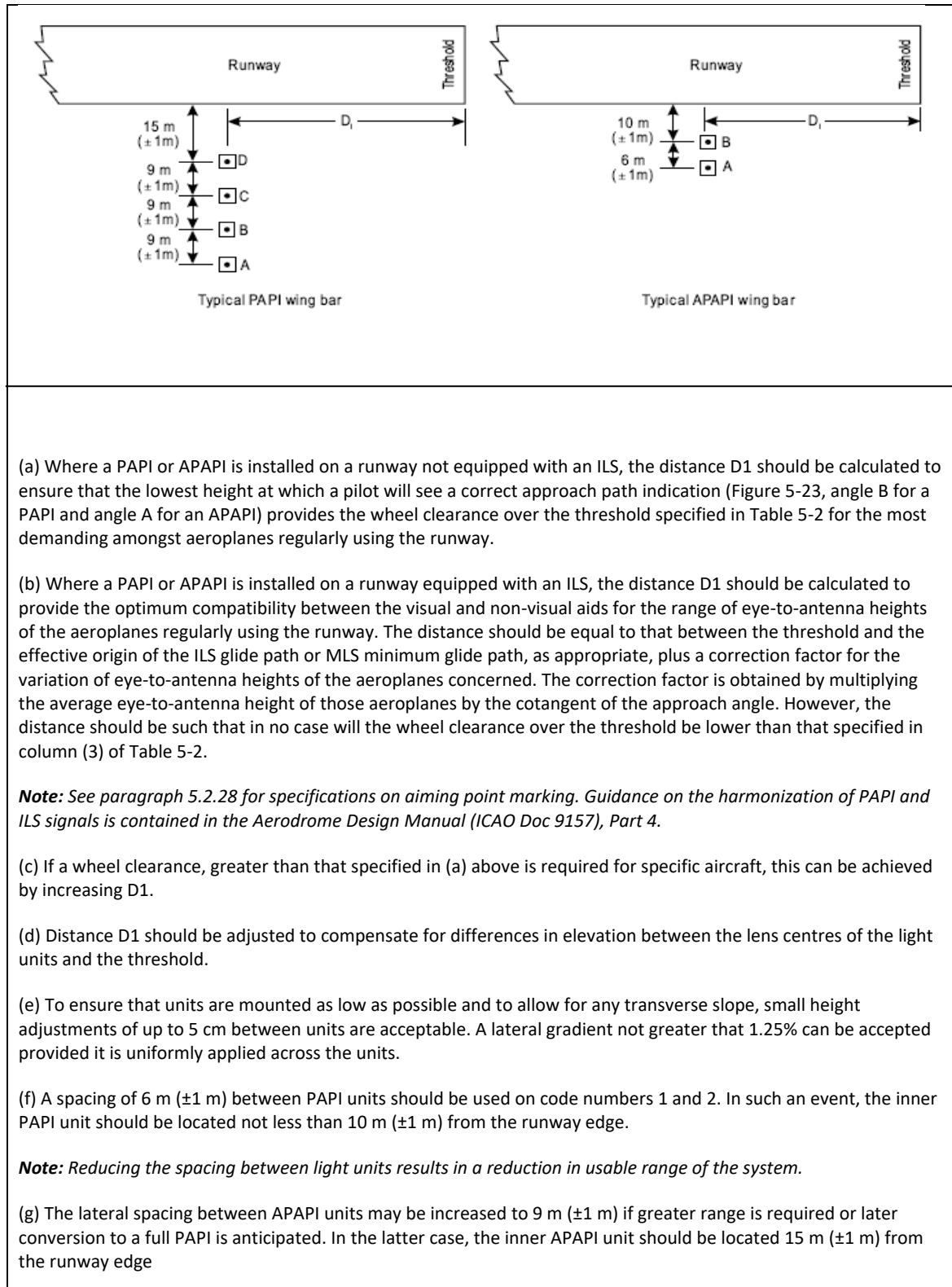
Figure 5-21 Installation of PAPI and APAPI
