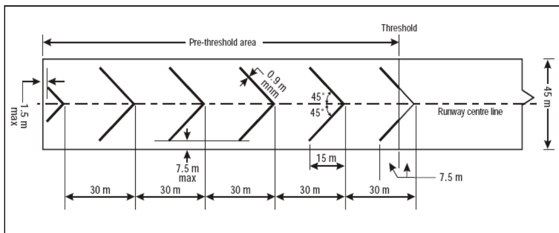
Figure 7-2 Pre-threshold marking
