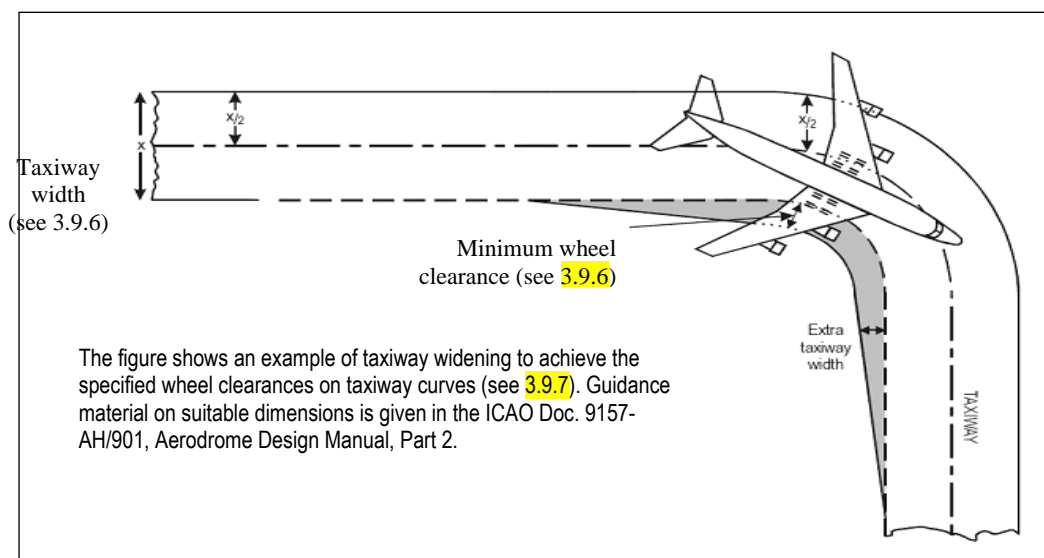
Figure 3-2. Taxiway curve
