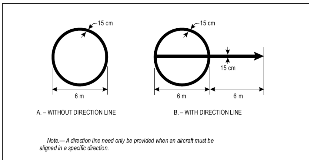
Figure 5-9. VOR aerodrome check point marking
