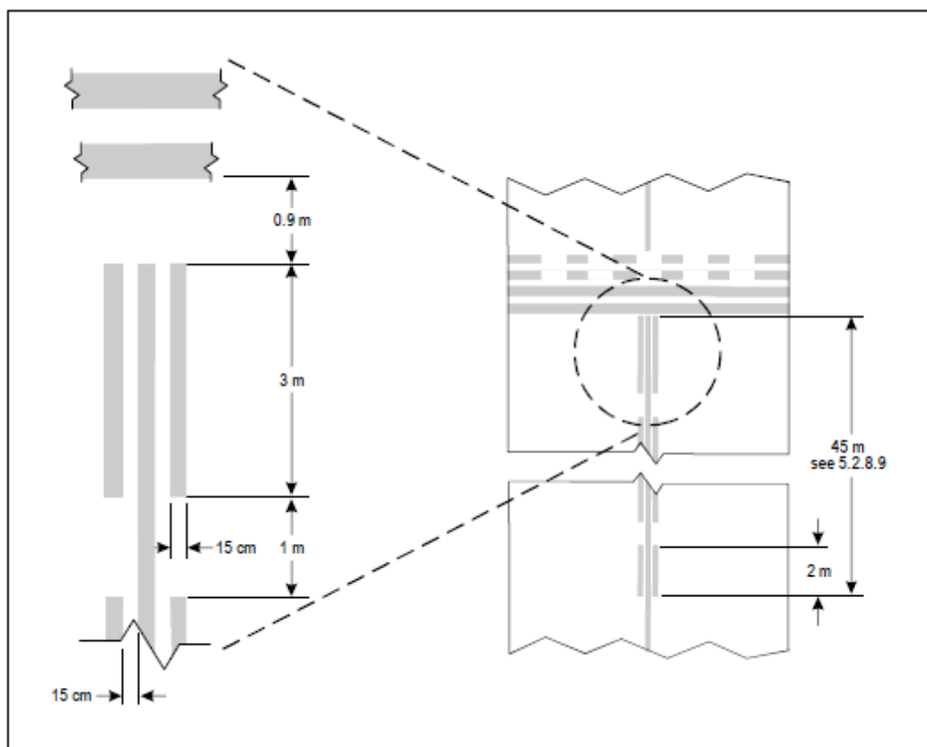
Figure 5-7. Enhanced taxiway centre line marking
