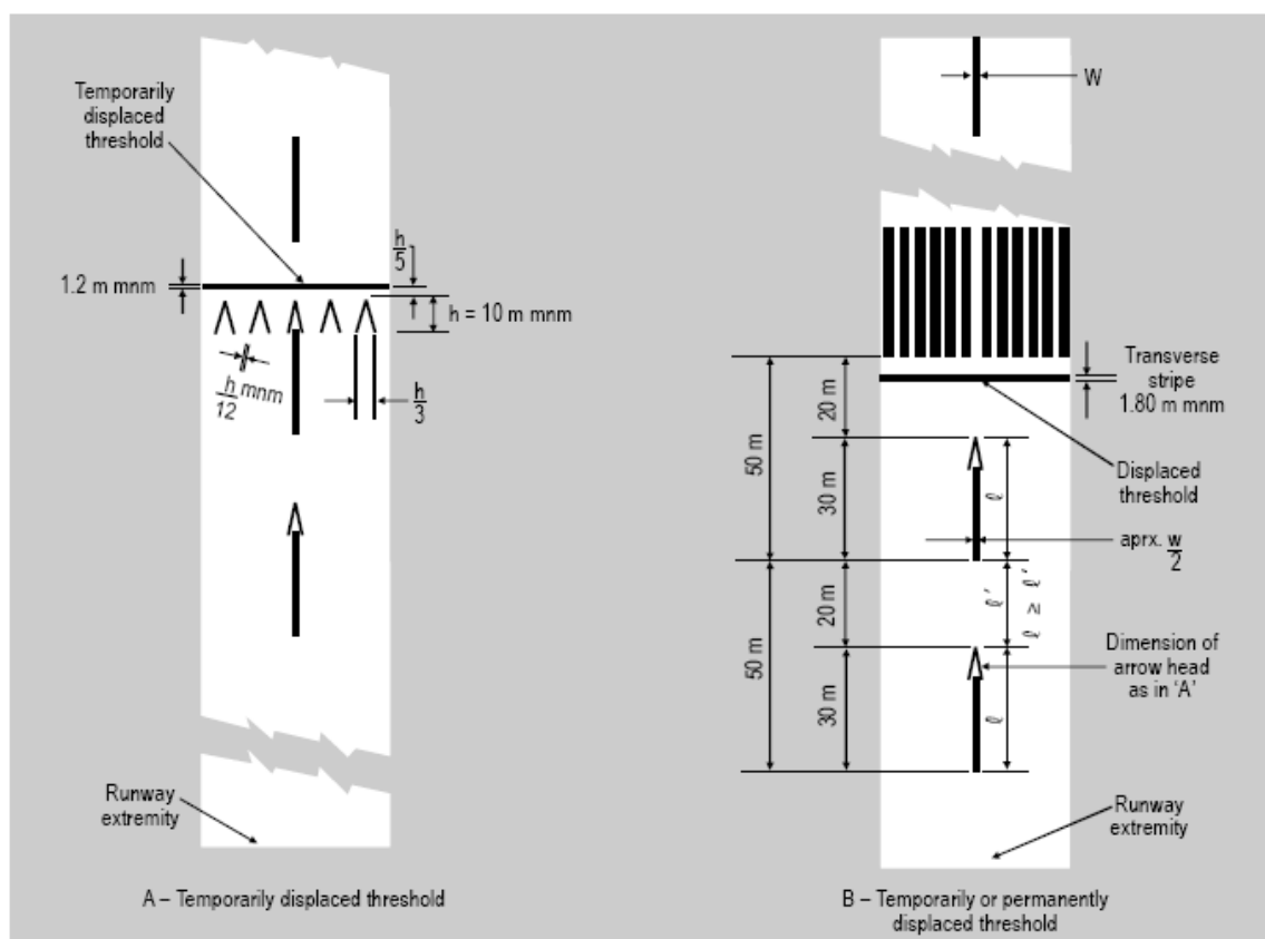
Figure 5-3. Displaced threshold markings
