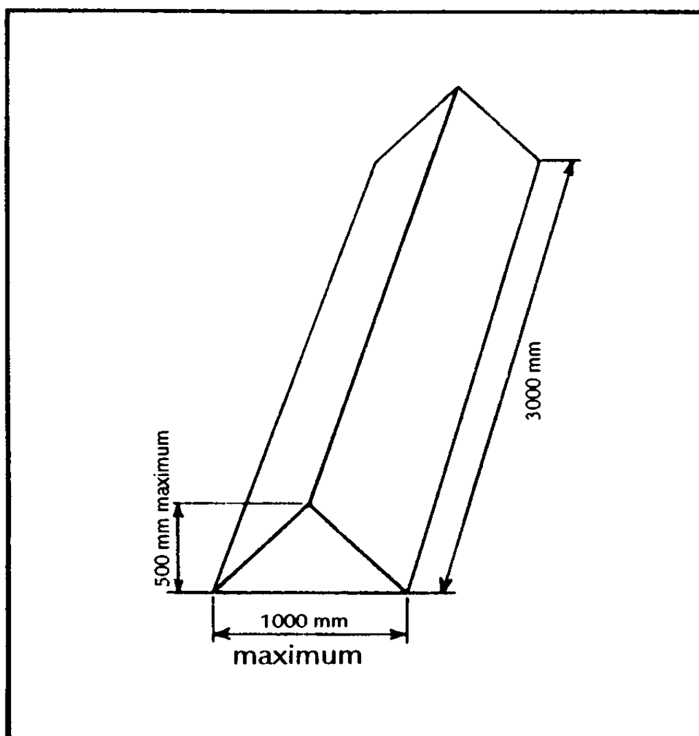
Figure 5-32 Marker Board
